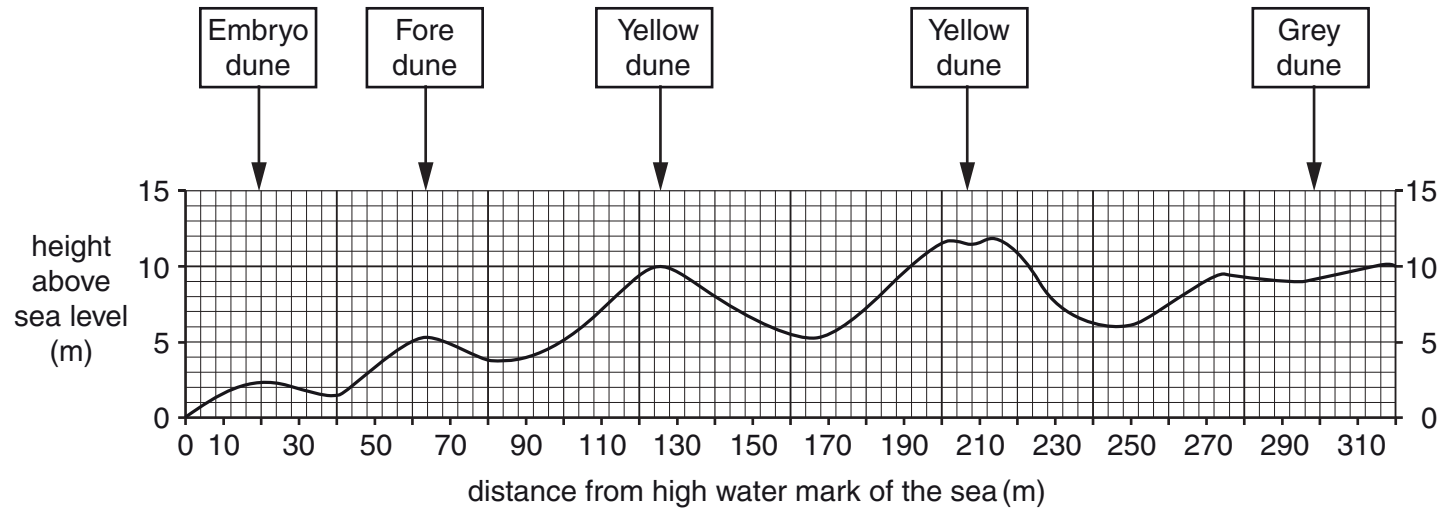
Transect profile across sand dunes
